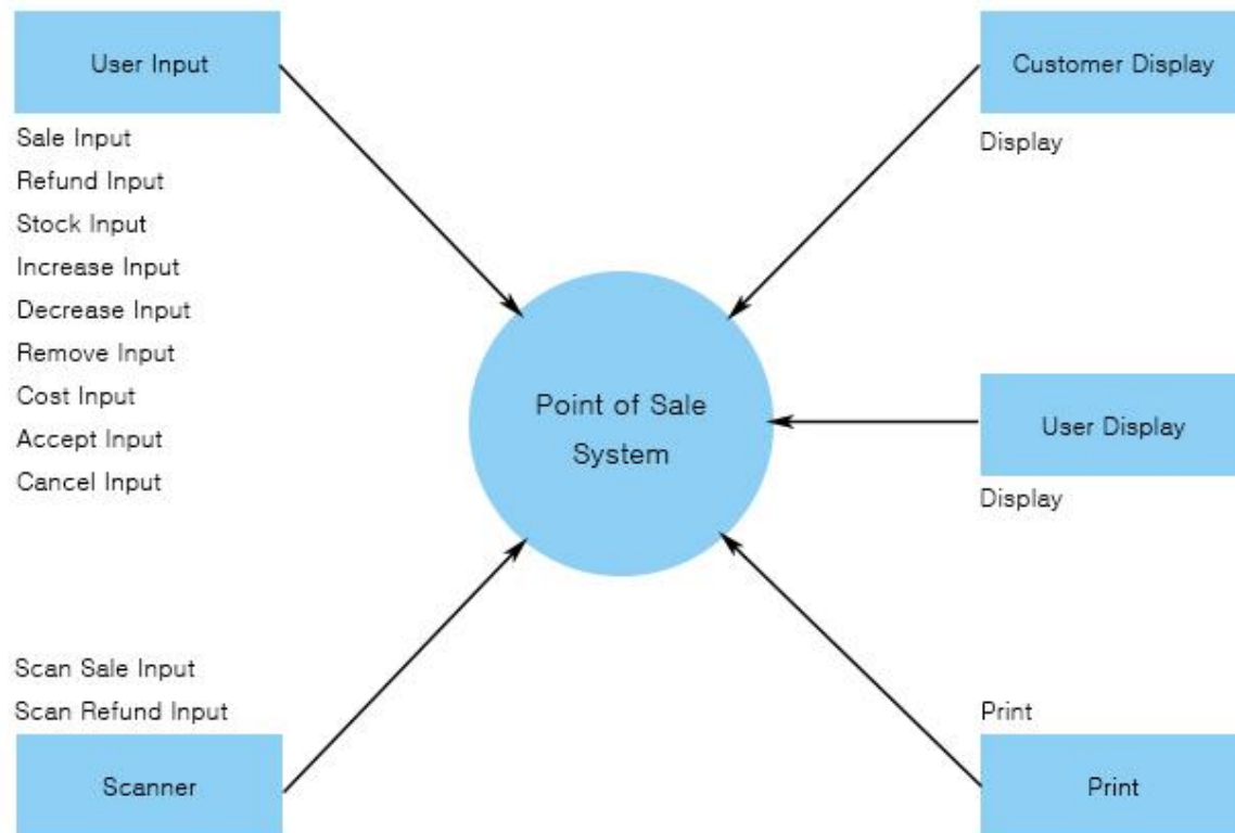
The System Context Diagram
